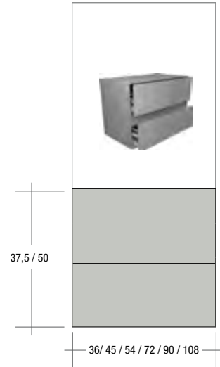
Base con 2 cassetti Cabinet with 2 drawers
